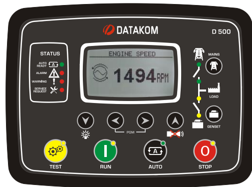
CONTROLLER
