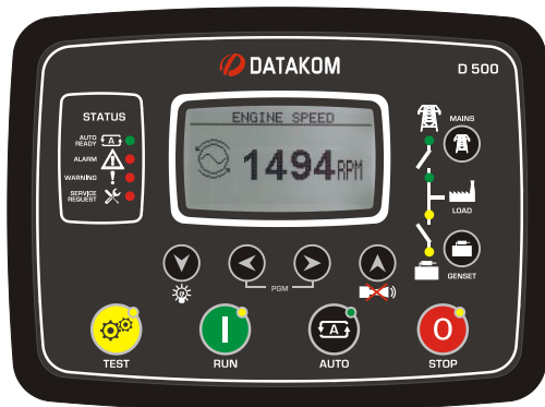
CONTROLLER
